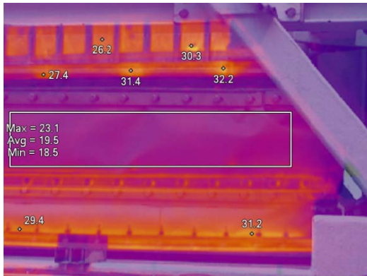
Visund 4tr. Compressor exhaust – bellows
