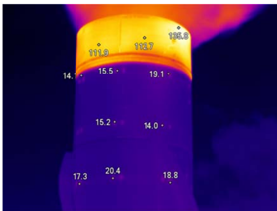
Visund 4 tr. Compressor exhaust outlet
