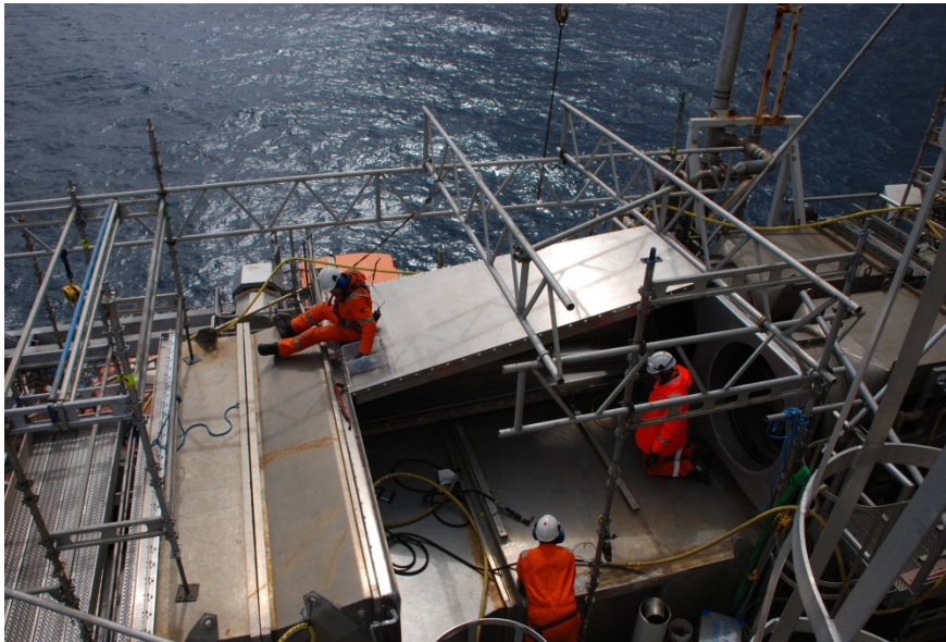
Modification on Visund 4 tr. Compressor ventilation inlet system – RS11.
